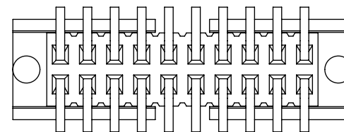
FIG 4 -DV-SA OPTION (SEE NOTES 6 & 7) FTS-106-02-XX-DV-SA SHOWN (DIFFERENT AS SHOWN, OTHERWISE SAME AS FIG 1) NOTE: 4 POSITIONS MUST BE ADDED TO PART CALLOUT TO ACHIEVE DIMS
