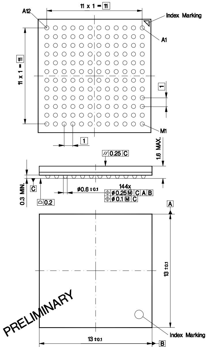
Figure 26 VINETIC®-2CPE (PEB 3332), VINETIC®-4M (PEB 3314), VINETIC®-4C (PEB 3394), VINETIC®-4S (PEB 3304)
