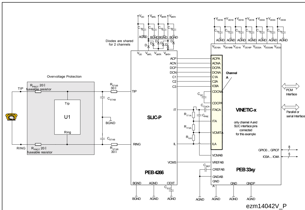
Figure 16 Application Circuit Internal Ringing (bal. & unbal.) for SLIC-P
