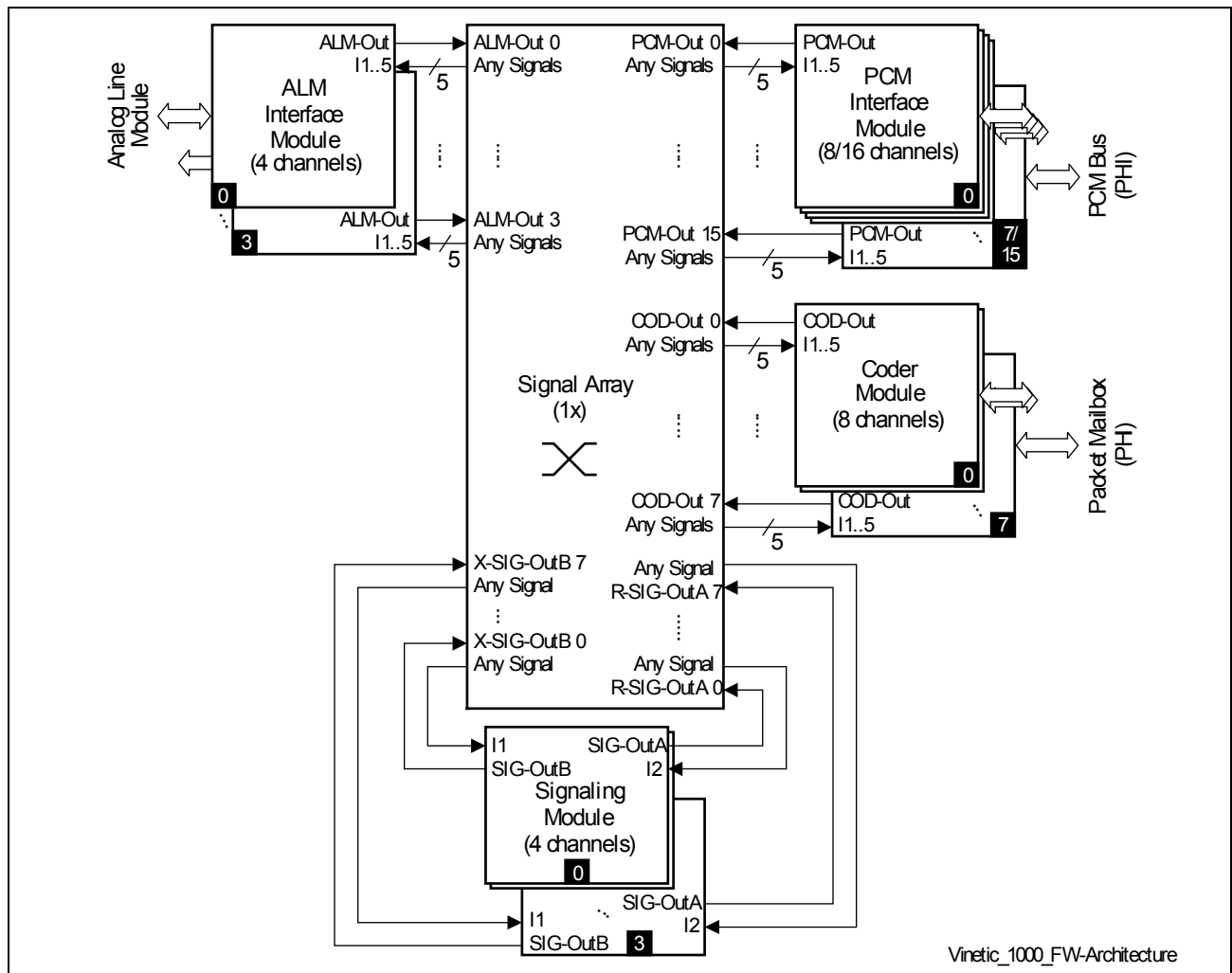
Figure 9 Module Concept
