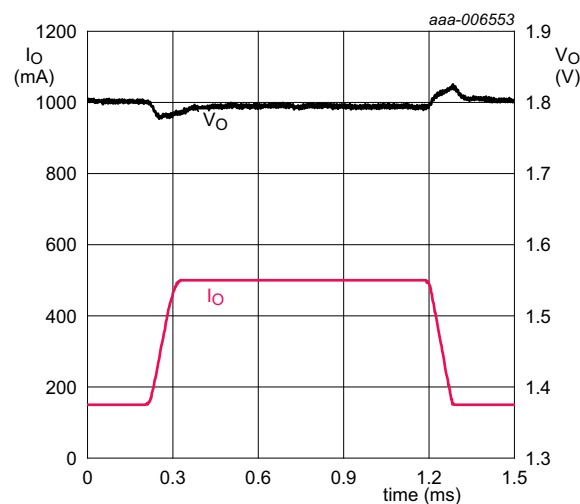
Fig 13. DC6M60xX6/18x: Load transient response
