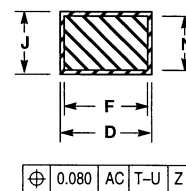
SECTION AE-AE
