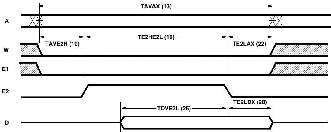
FIGURE 6. WRITE CYCLE III: EARLY WRITE - CONTROLLED BY \overline{E2}
