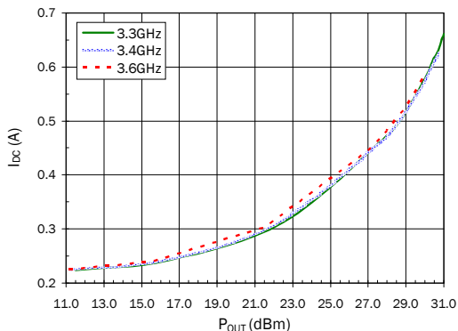
DC Supply Current ( I_{DC} ) versus P_{OUT} , T=25^\circ C
