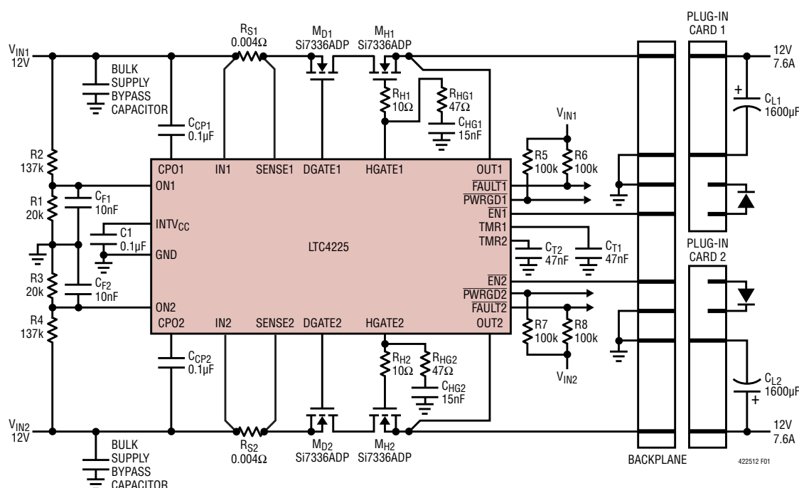
Figure 1. \mu TCA Application Supplying 12V Power to Two \mu TCA Slots
