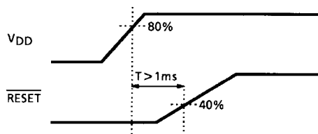
Figure 5 Power On Reset Timing
