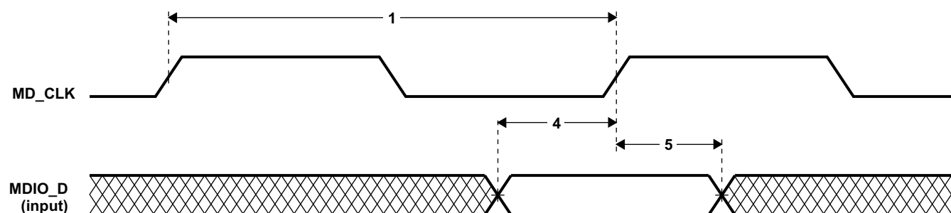
Figure 6-53. MDIO Input Timing
