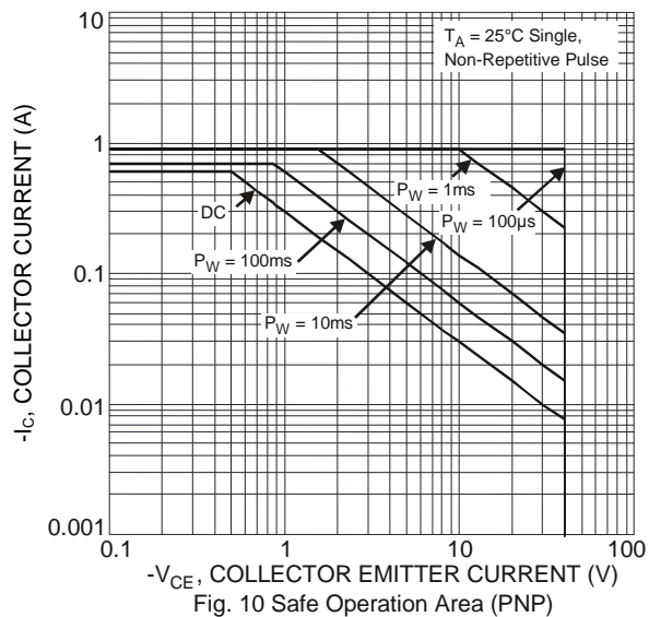
Fig. 10 Safe Operation Area (PNP)
