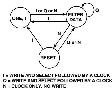
Figure 11. State Transition Diagram of AD9761 Digital Interface
