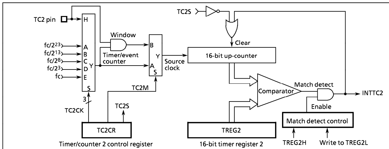
Figure 2-26. Timer/Counter 2 (TC2)
