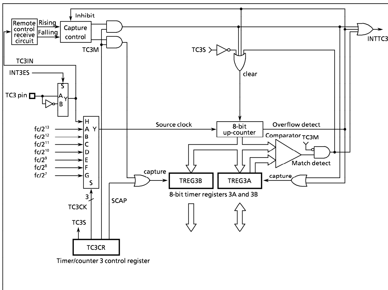
Figure 2-29. Timer/Counter 3 (TC3)
