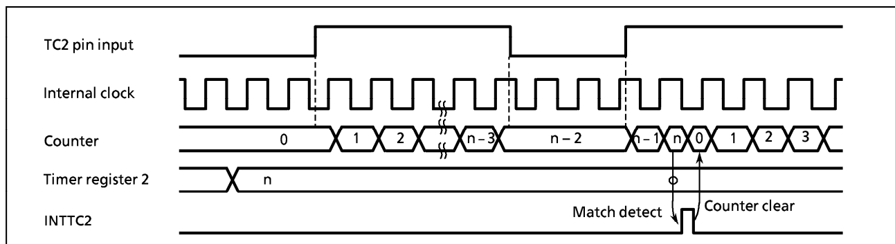
Figure 2-28. Window Mode Timing Chart
