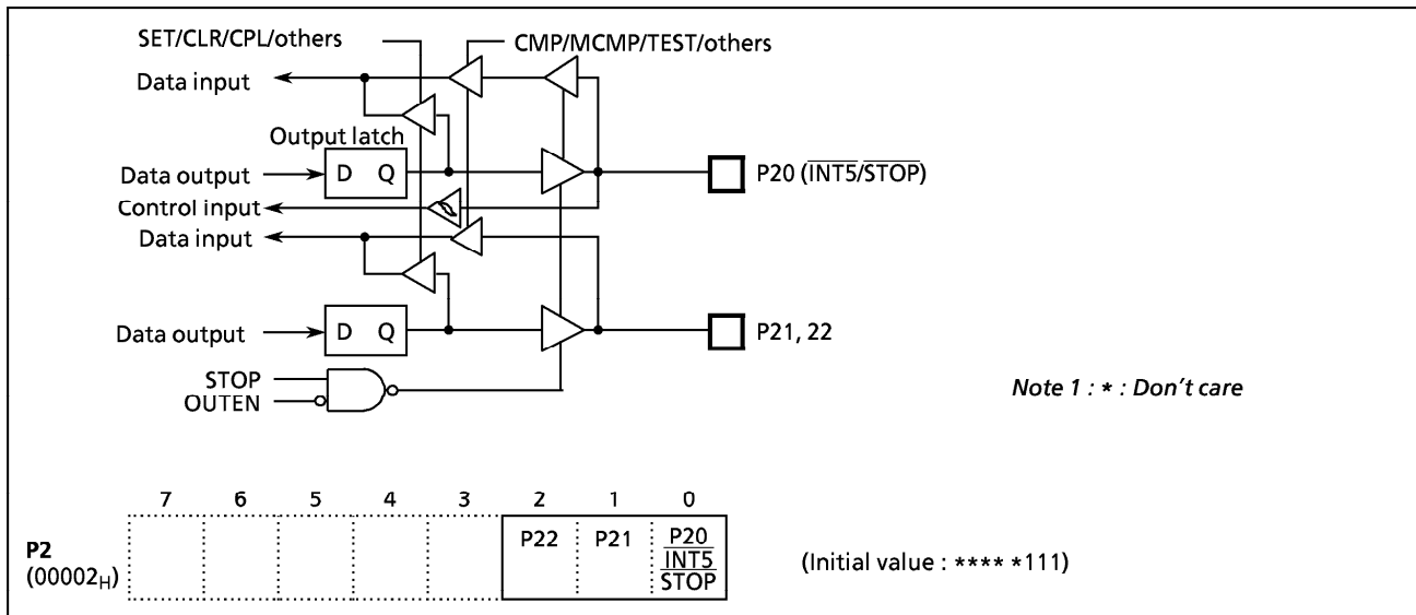
Figure 2-5. Port P2
