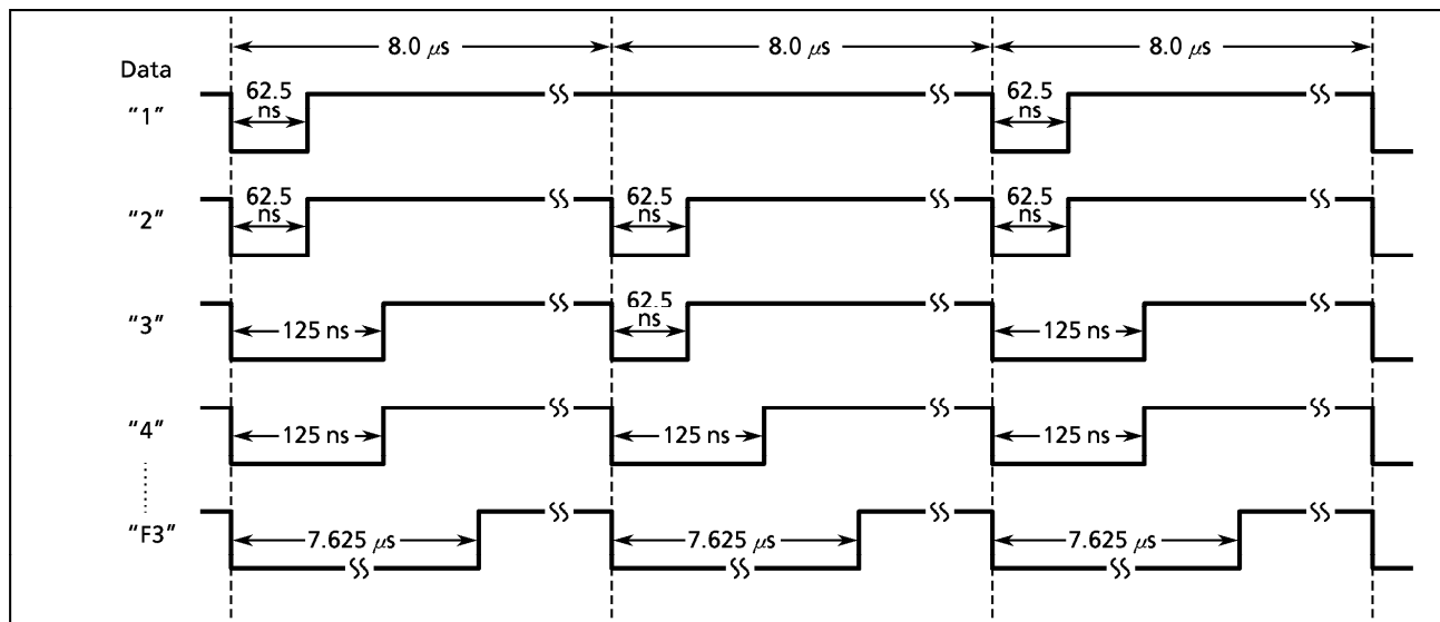
Figure 2-93. 6-Bit Mode
