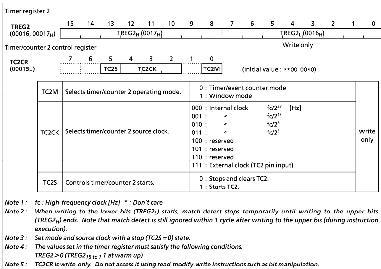
Figure 2-27. Timer/Counter 2 Timer Register and Control Register
