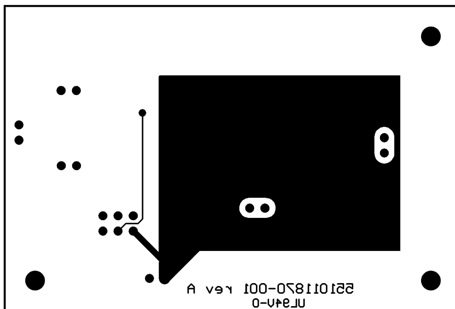
Figure 38. Bottom Layer
