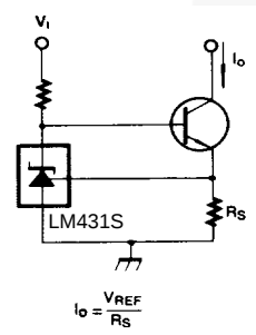
Figure 19. Constant-Current Sink
