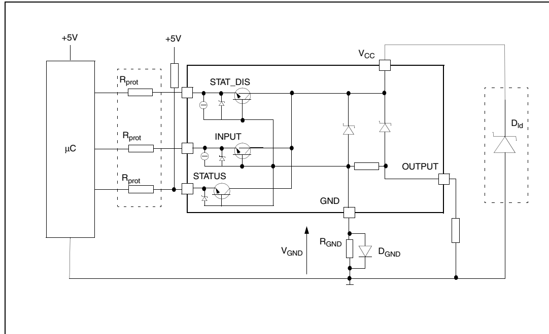
Figure 27. Application schematic
