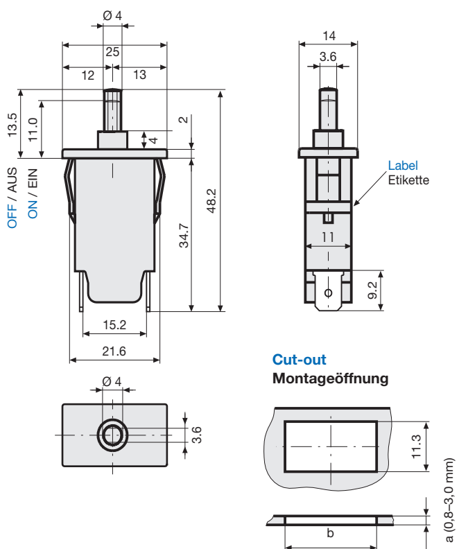
T11-611 ≤7,5 A
