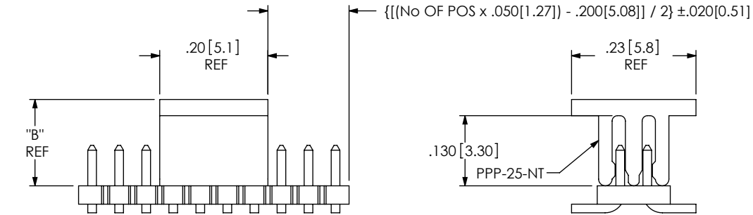
(USE PPP-25-NT FOR TAPE AND REEL PACKAGING ONLY) FIG 4 -DV-SA OPTION (SEE NOTES 6 & 7) FTS-106-02-XX-DV-SA SHOWN (DIFFERENT AS SHOWN, OTHERWISE SAME AS FIG 1) NOTE: 4 POSITIONS MUST BE ADDED TO PART CALLOUT TO ACHIEVE DIMS
