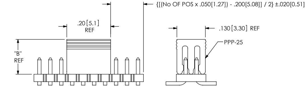
FIG 5 -DV-P OPTION (SEE NOTES 6 & 7) FTS-110-02-XX-DV-P SHOWN (DIFFERENT AS SHOWN, OTHERWISE SAME AS FIG 1)
