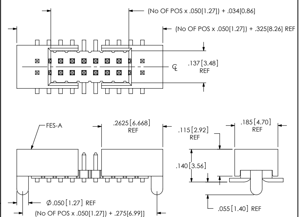
FIG 3 -DV-S OPTION (SEE NOTES 6 & 7) FTS-110-02-XX-DV-S SHOWN (DIFFERENT AS SHOWN, OTHERWISE SAME AS FIG 1) NOTE: 4 POSITIONS MUST BE ADDED TO PART CALLOUT TO ACHIEVE DIMS (NOT AVAILABLE WITH -A OPTION; ORDER -SA FOR ALIGNMENT PIN WITH SHROUD)
