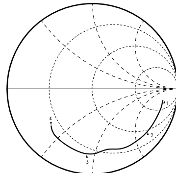
Figure 18. LMX243x TSSOP FinRF Input Impedance
