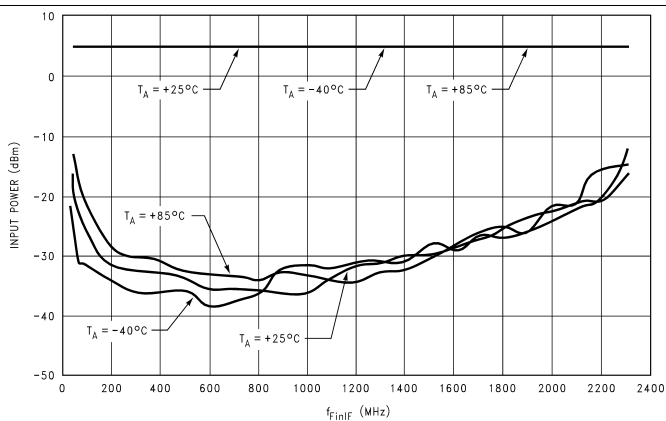
Figure 10. LMX2433 FinIF Input Power vs Frequency
