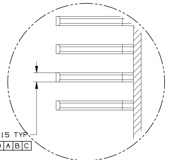
DETAIL N SCALE 5:1
