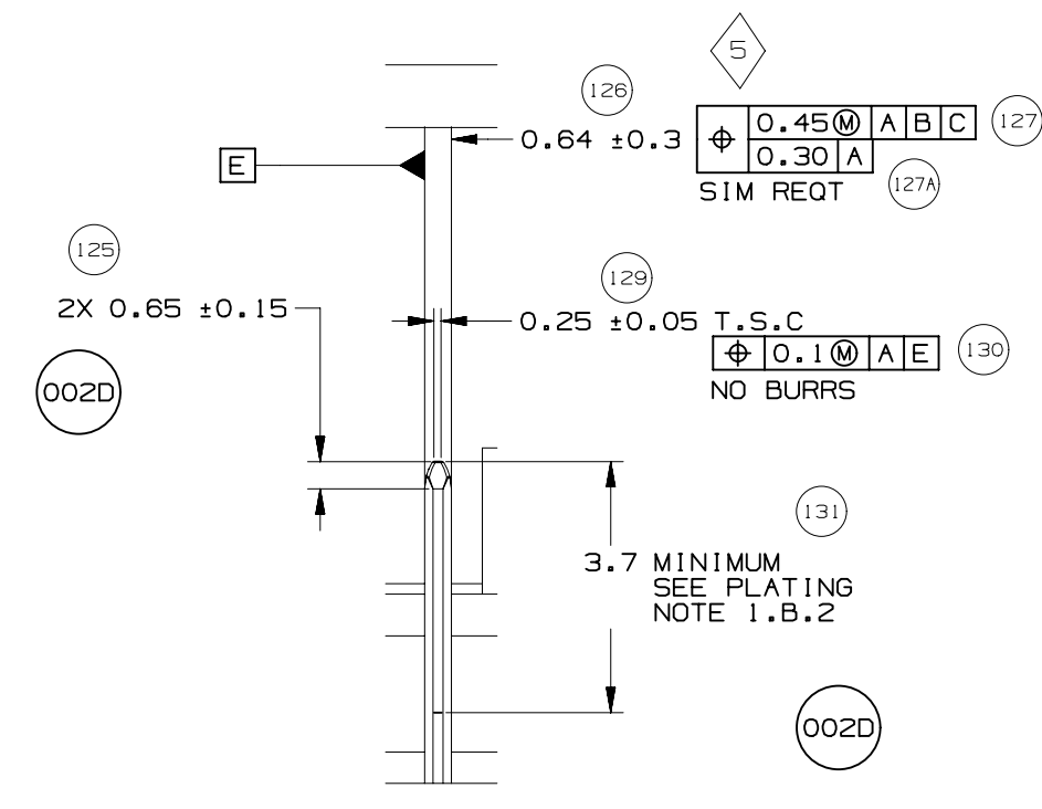
SECTION U-U
