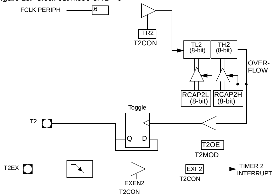
Figure 15. Clock-out Mode C/\overline{T2} = 0
