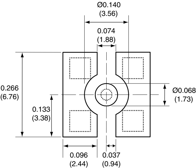
RECOMMENDED FOOTPRINT
