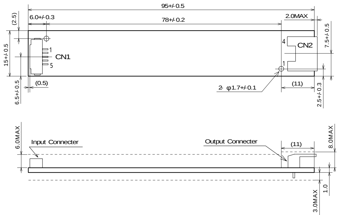
Fig.3 Dimensional Outline
