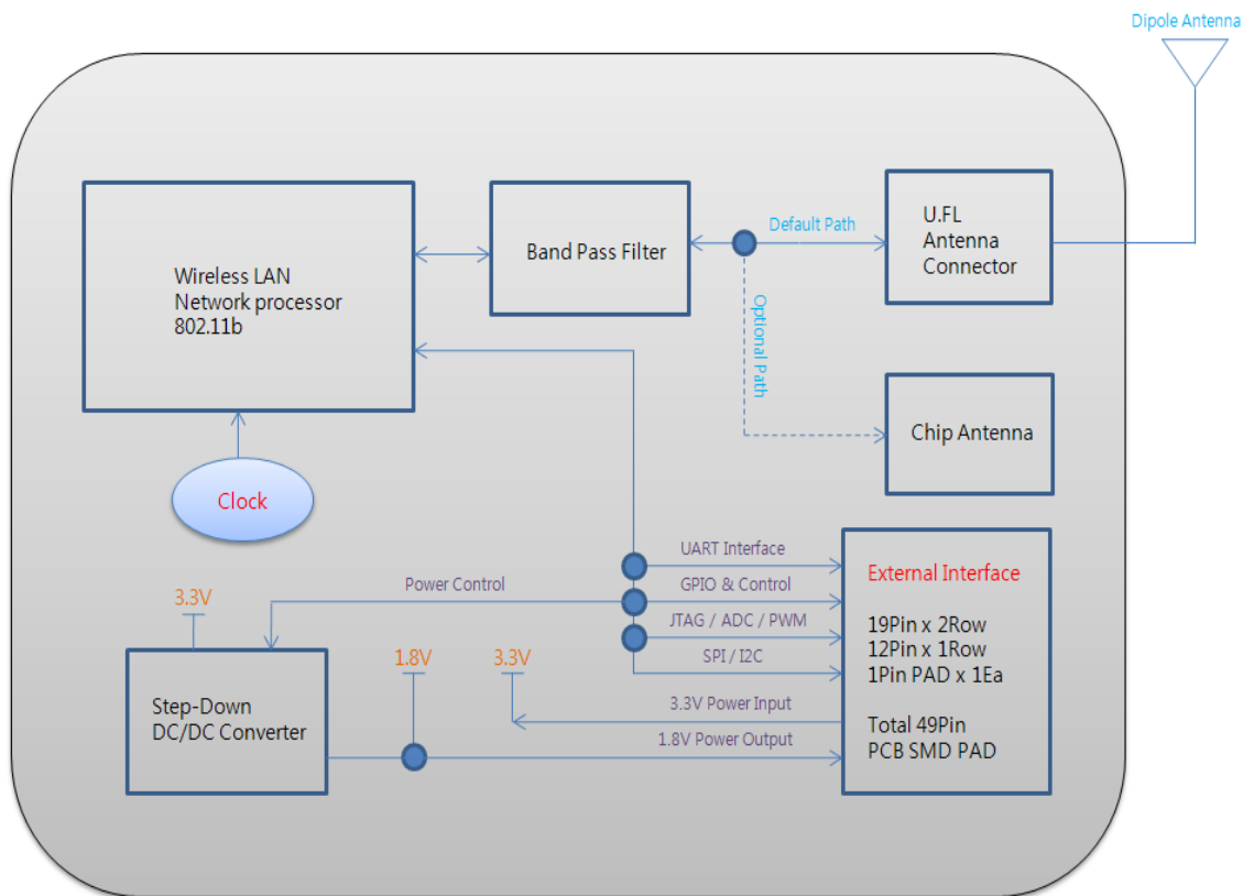
Figure 2. Block Diagram
