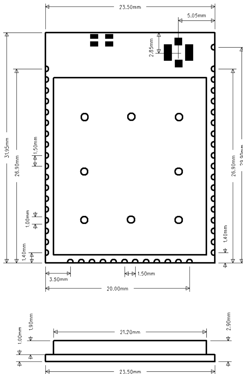
Figure 4. Module dimension
