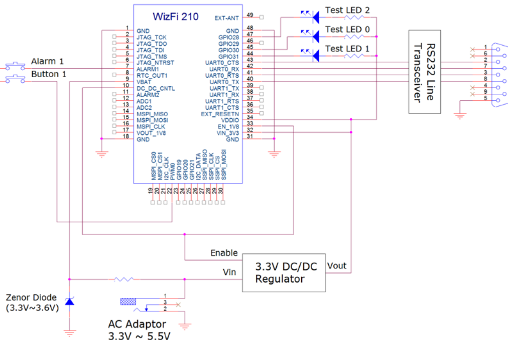
Figure 7. V_{IN} = AC Adaptor, Standby support
