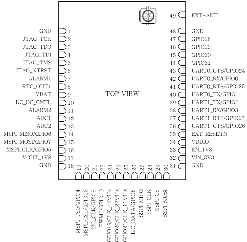
Figure 3. Pin description
