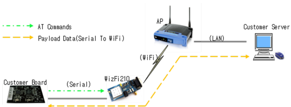
Figure 1. Basic Diagram
