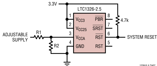
Dual Supply Monitor (3.3V Plus Adj)
