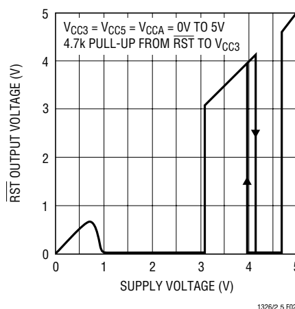
Figure 2. \overline{\text{RST}} Voltage vs Supply Voltage
