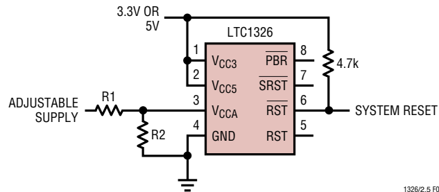
Dual Supply Monitor (3.3V or 5V Plus Adj)
