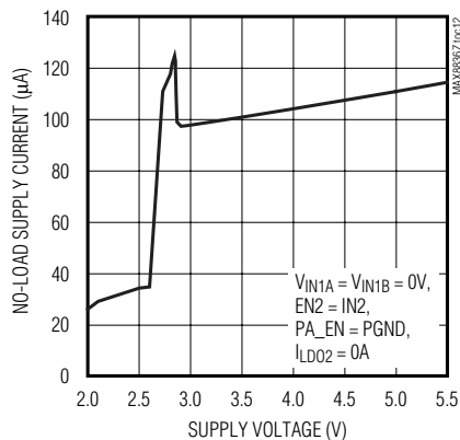
LD02 SUPPLY CURRENT vs. SUPPLY VOLTAGE
