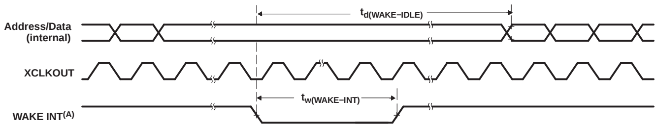
Figure 6-11. IDLE Entry and Exit Timing
