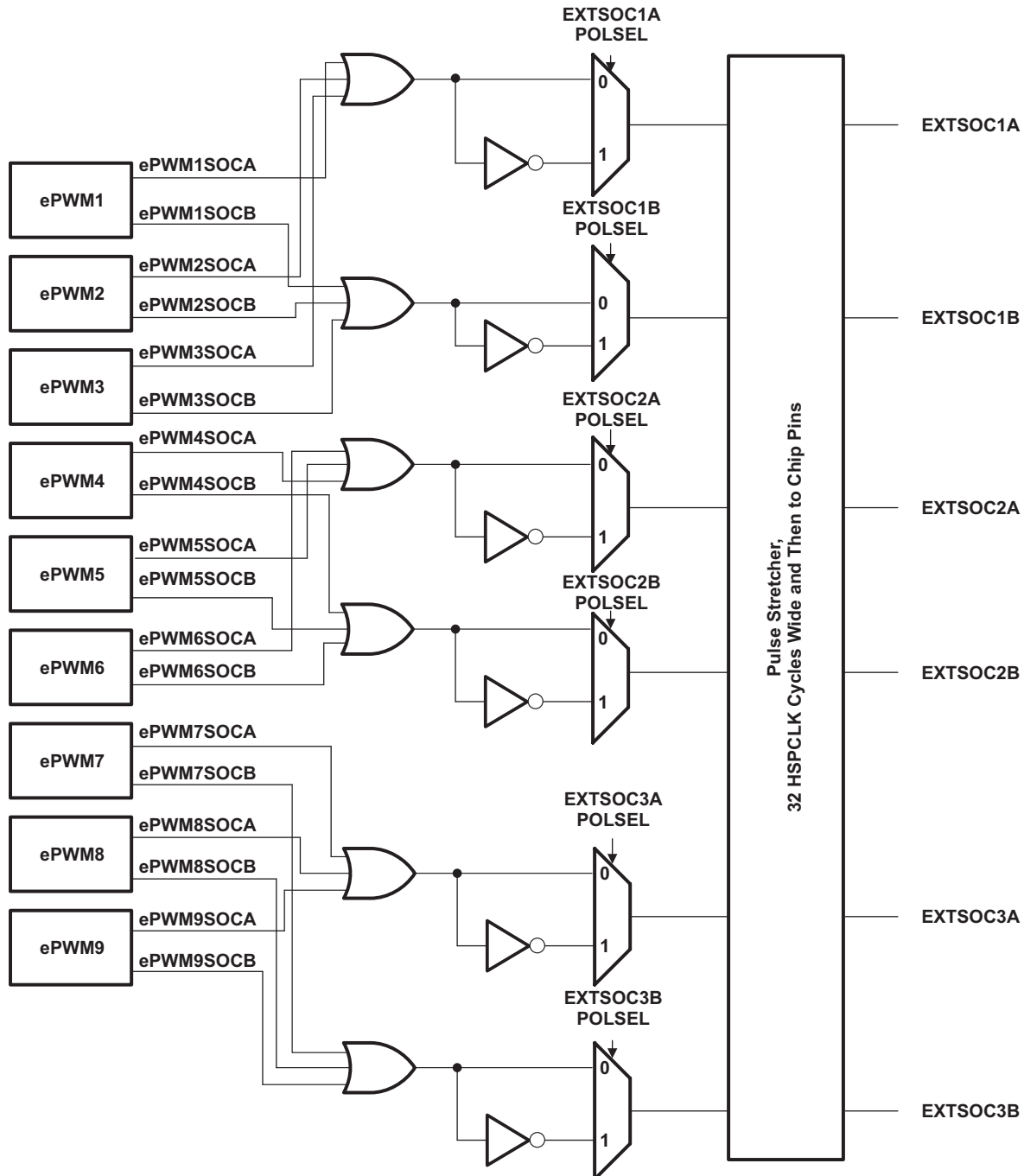
Figure 4-8. External ADC Interface
