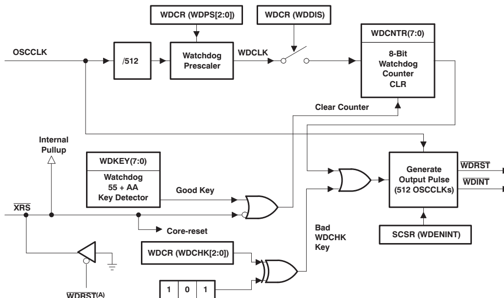
Figure 3-13. Watchdog Module
