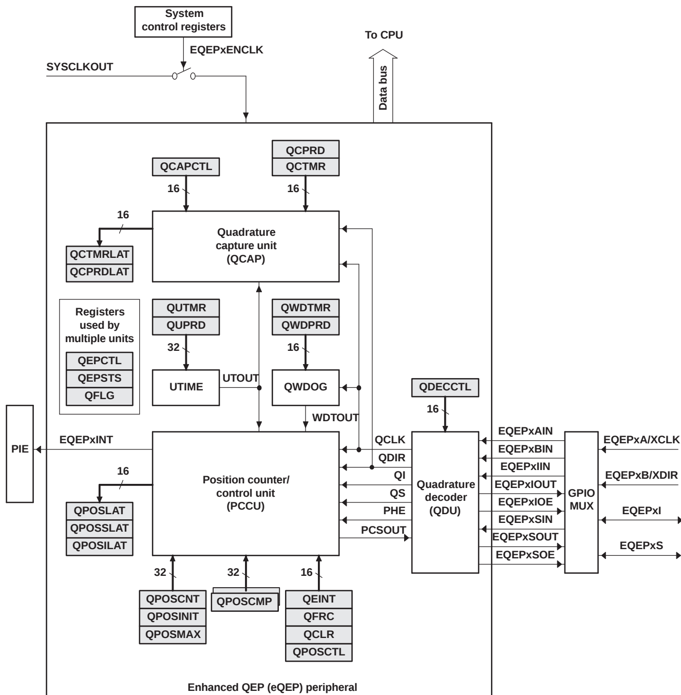
Figure 4-7. eQEP Functional Block Diagram
