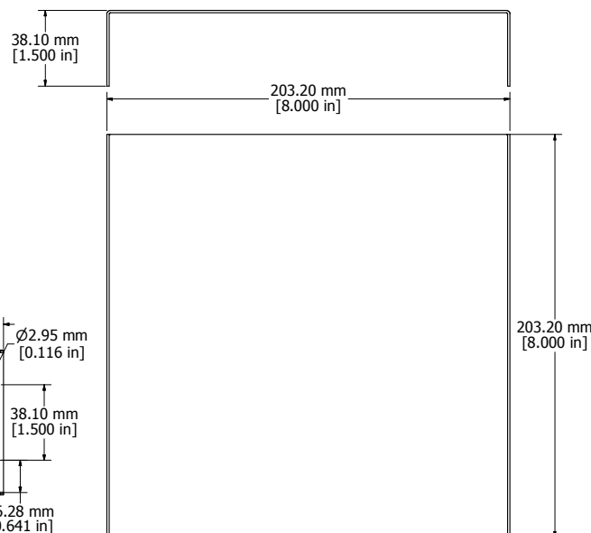
BOTTOM/TOP ENCLOSURE
