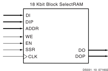
Figure 30: 18 Kbit Block SelectRAM Memory in Single-Port Mode
