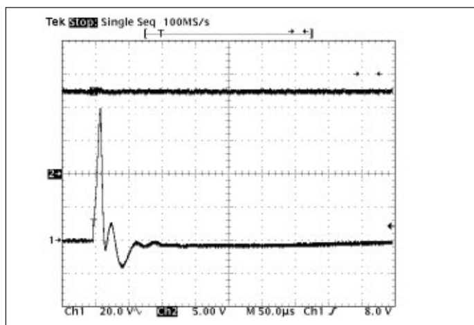
Figure 2 – Transient Immunity: M-FIAM5 output response to an input transient.
