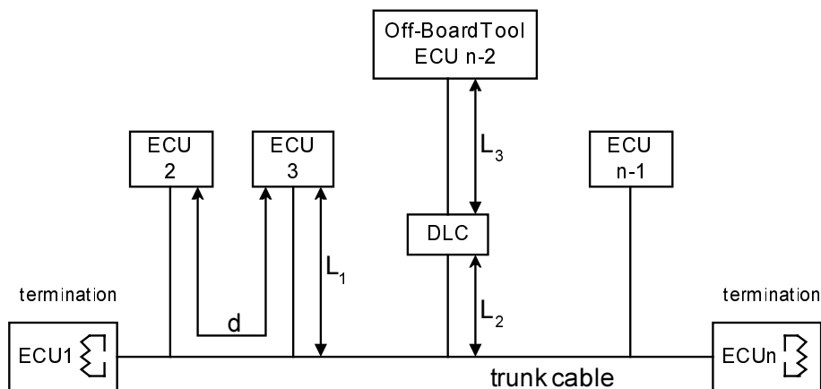
Figure 9.2: Topology requirements of SAE J2284
