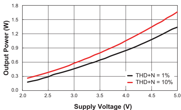
Output Power vs. Supply Voltage ( f = 1\text{kHz} ; R_L = 8\Omega )
