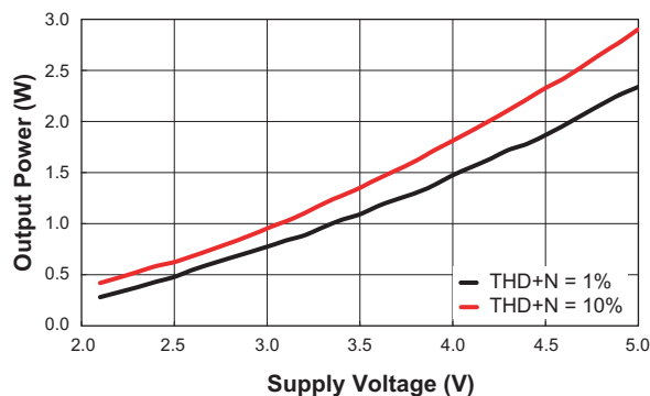
Output Power vs. Supply Voltage ( f = 1\text{kHz} ; R_L = 4\Omega )
