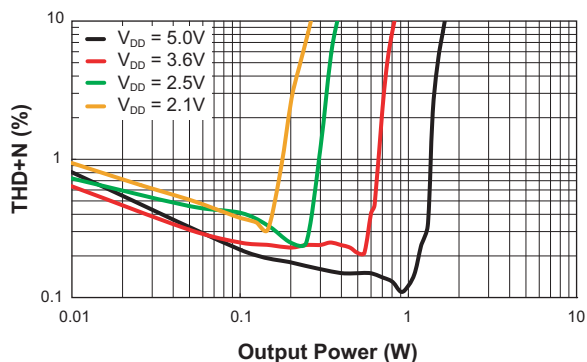
THD+N vs. Output Power ( f = 1\text{kHz} ; R_L = 8\Omega )
