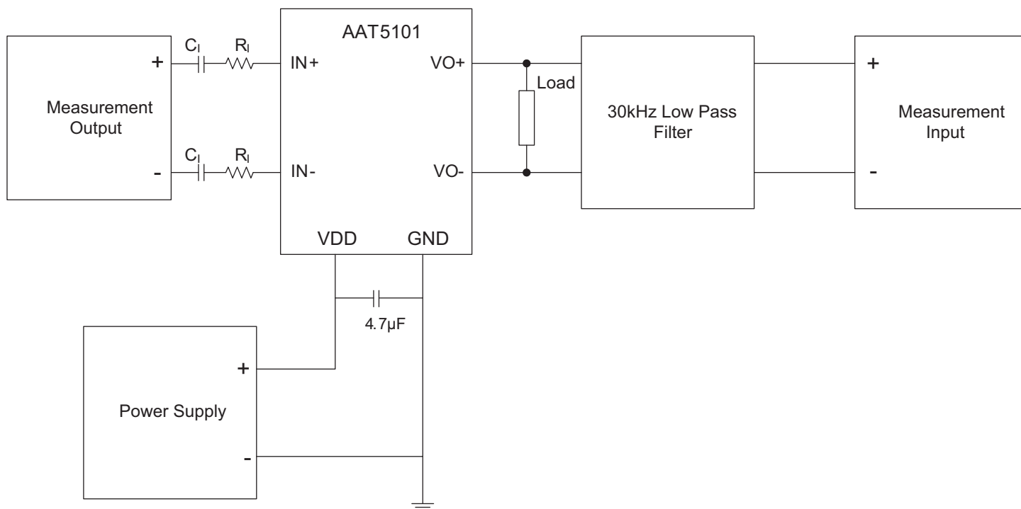
Test Set-up for Typical Characteristics Graphs.
