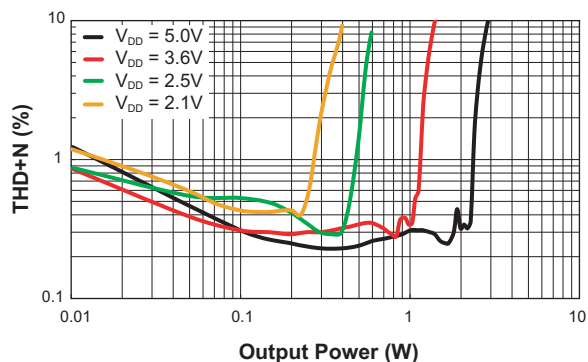
THD+N vs. Output Power ( f = 1\text{kHz} ; R_L = 4\Omega )
