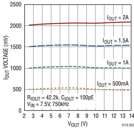
I_{OUT} Voltage vs V_{OUT}
