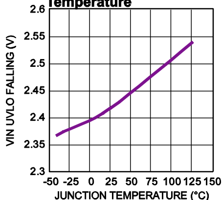
V_{IN} UVLO Falling Threshold vs. Temperature
