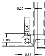
Hinge Detail
