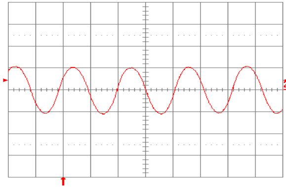
Fig. 2.5V.13: Input reflected-ripple current, i_e (100 mA/div.), measured at input terminals at full rated load current and V_{in} = 48 V. Refer to Fig. 2.5V.12 for test setup. Time scale: 1 \mu s/div.
