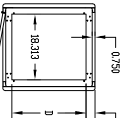
TOP VIEW (LESS TOP COVER & TOP COWLS)
