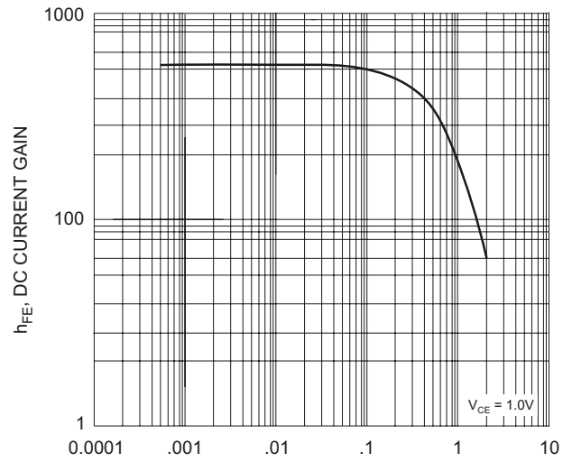
Fig. 2, Typical DC Current Gain vs Collector Current
