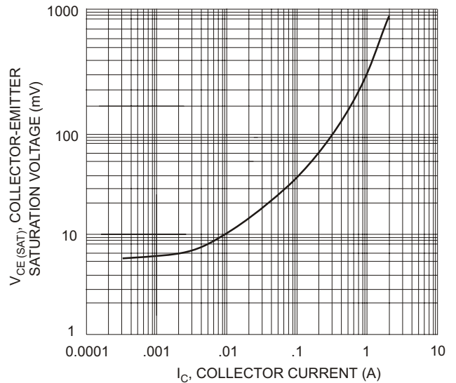
Fig. 4, Collector Saturation Voltage vs Collector Current
