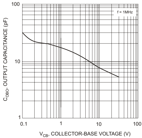
Fig. 3, Output Capacitance vs. Collector-Base Voltage
