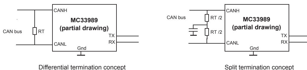
Figure 37. Bus Termination
