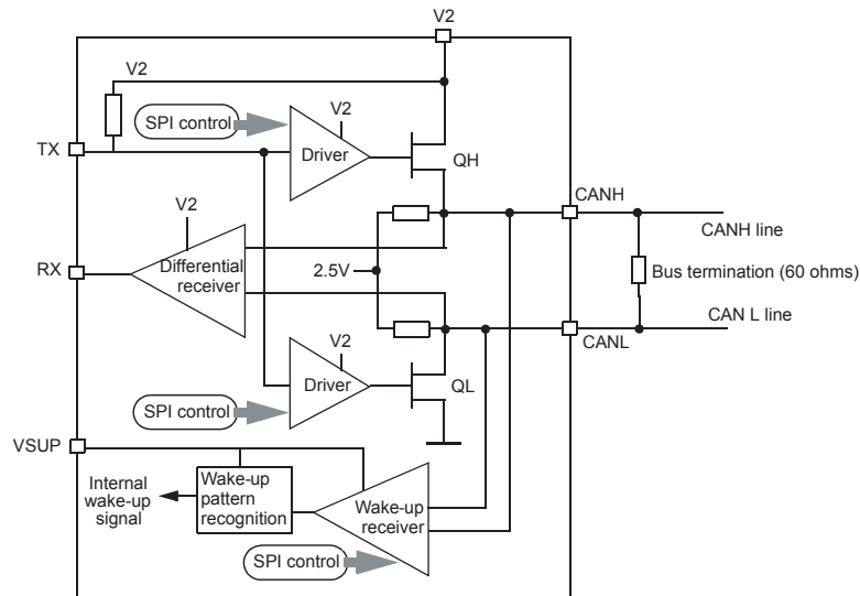
Figure 34. 33989 CAN Interface
