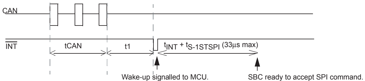
Figure 30. CAN Wake-up
