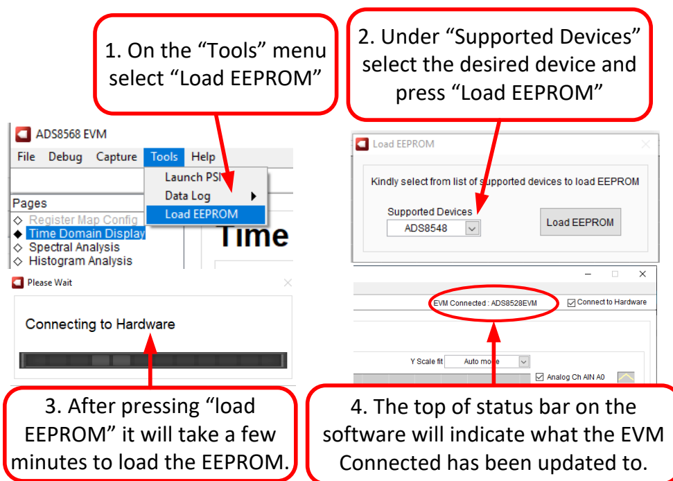
Figure 7-2. Configure EEPROM and Software for New Device
