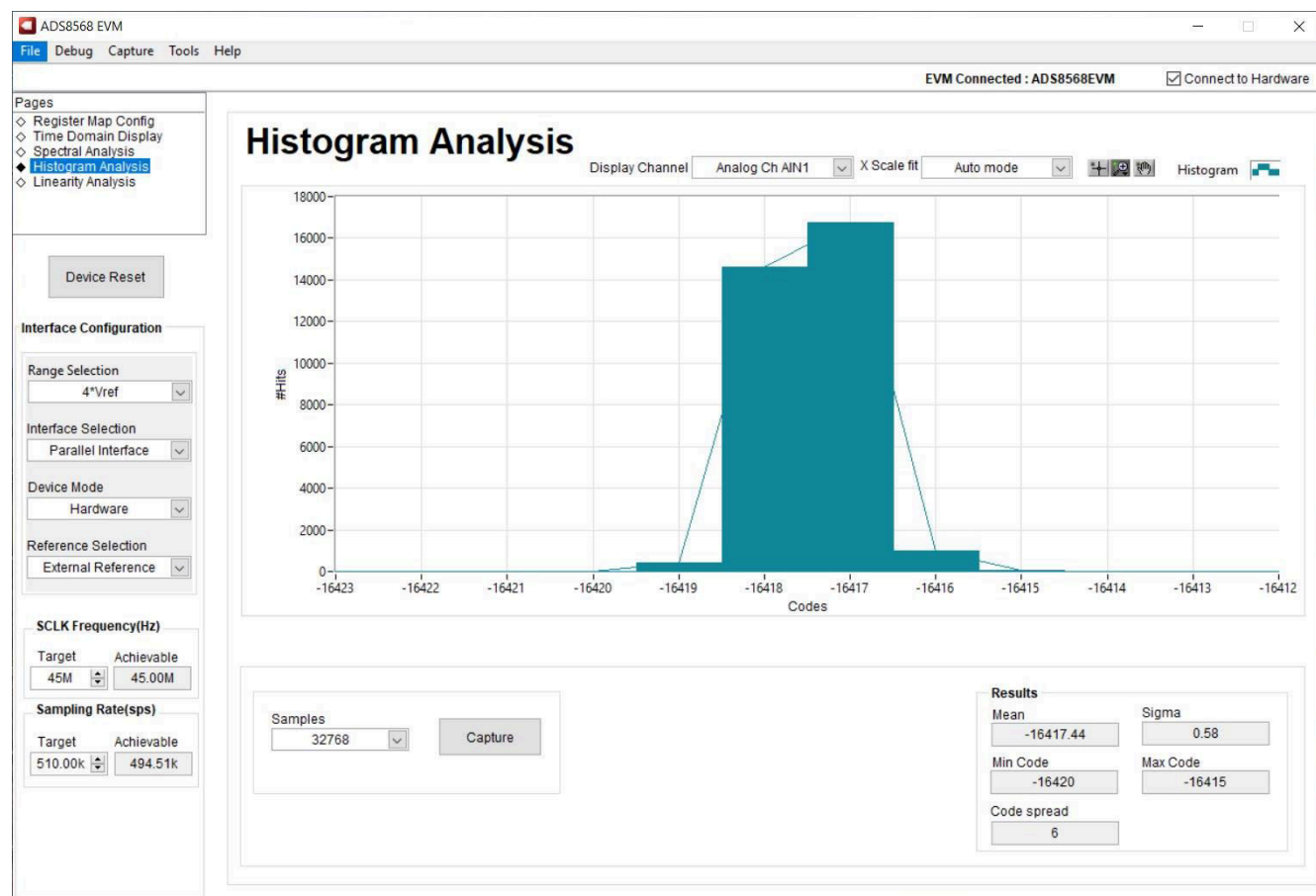
Figure 6-6. Histogram Display
