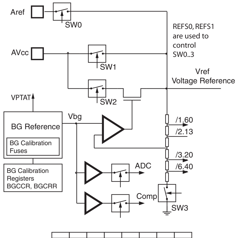
Figure 15-1. Reference circuitry.
