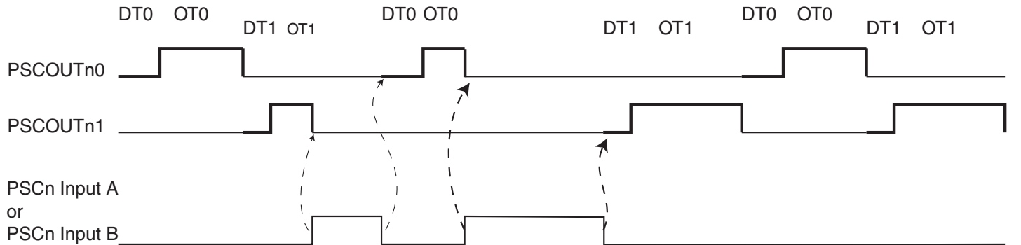
Figure 13-24. PSCR behavior versus PSCR Input A in Fault Mode 6.
