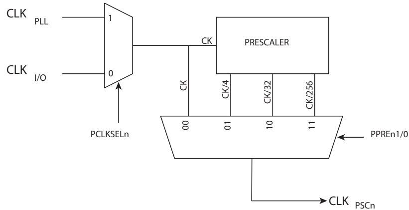
Figure 12-42. Clock selection.
