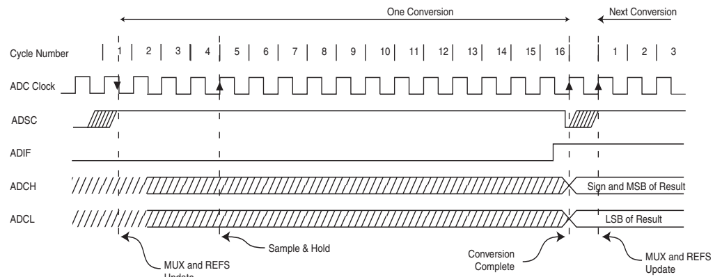
Figure 17-5. ADC timing diagram, single conversion.
