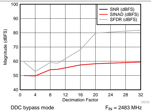
Figure 6. SNR, SINAD, SFDR vs Decimation Setting
