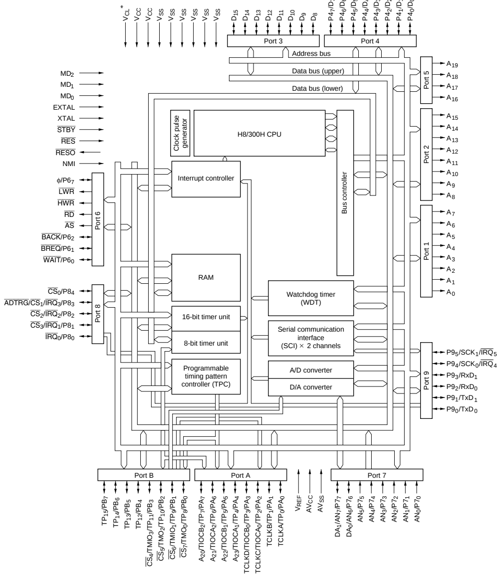
Figure 1.1 Block Diagram
