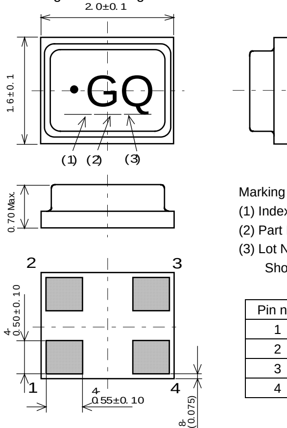
Fig.2 Package dimensions (in mm)
