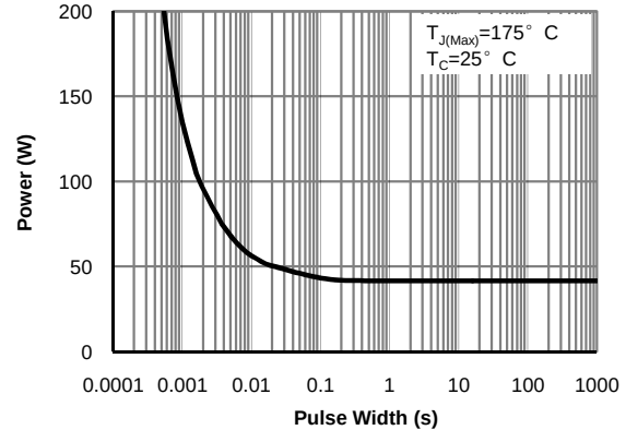
Figure 10: Single Pulse Power Rating Junction-to-Case for AOT2618L and AOB2618L (Note F)
