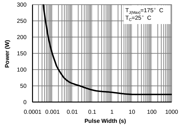
Figure 13: Single Pulse Power Rating Junction-to-Case for AOTF2618L (Note F)
