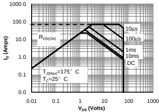
Figure 9: Maximum Forward Biased Safe Operating Area for AOT2618L and AOB2618L (Note F)
