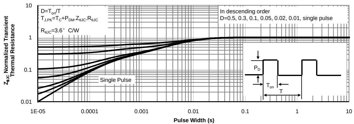
Figure 11: Normalized Maximum Transient Thermal Impedance for AOT2618L and AOB2618L (Note F)
