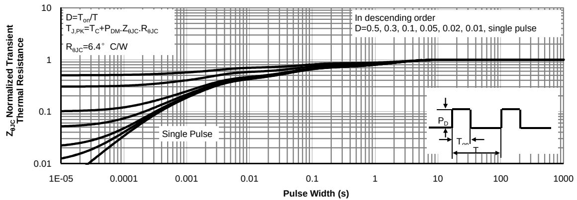
Figure 14: Normalized Maximum Transient Thermal Impedance for AOTF2618L (Note F)
