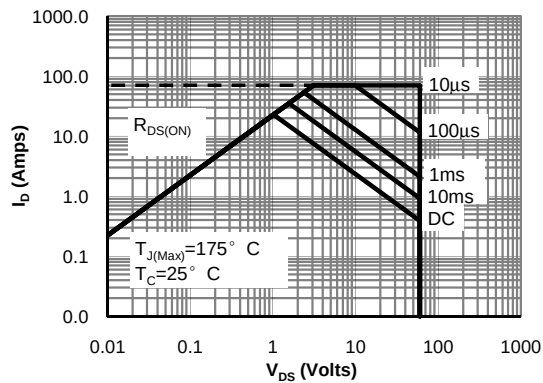
Figure 12: Maximum Forward Biased Safe Operating Area for AOTF2618L
