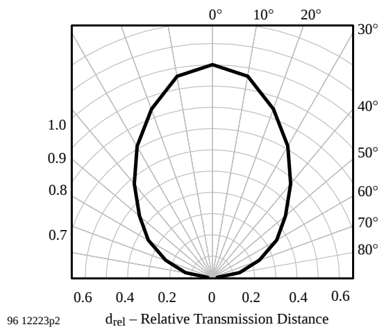
Figure 12. Directivity tsop
