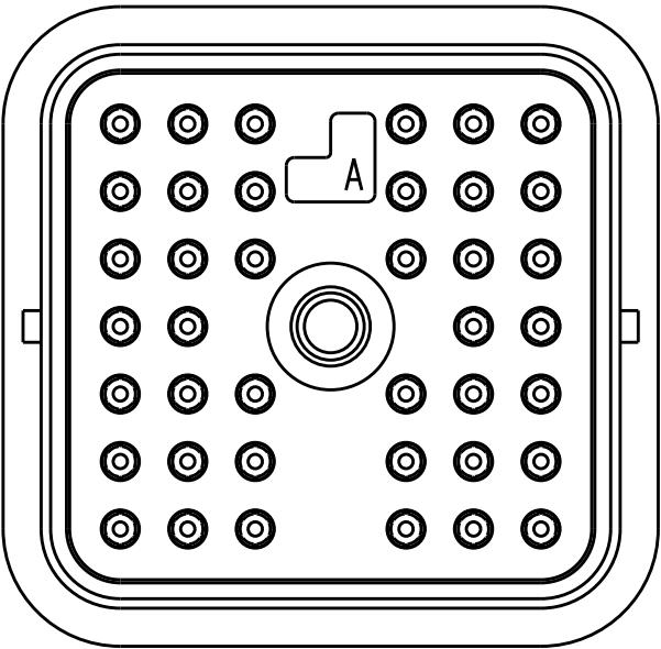
AEC16-40SAE-E019 KEY 'A'
