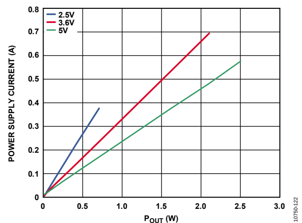
Figure 22. Power Supply Current vs. P_{OUT} , 8 \Omega
