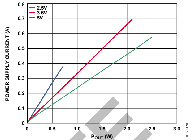
Figure 20. Power Supply Current vs. P_{OUT} , 4 \Omega
