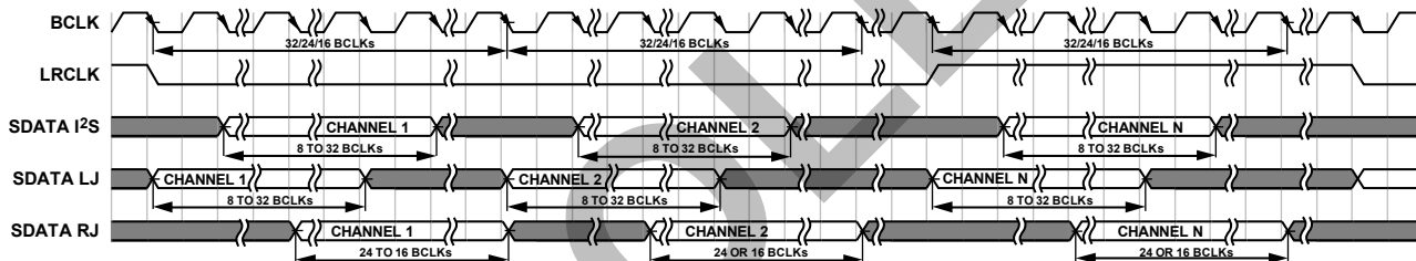
Figure 27. TDM Modes with 50% Duty Cycle LRCLK
