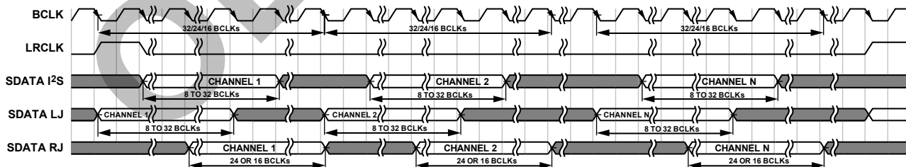
Figure 28. TDM Modes with Pulse Mode LRCLK
