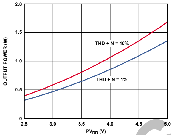
Figure 18. Maximum Output Power vs. PV_{DD} ( f_{IN} = 1 kHz, R_L = 8 \Omega )
