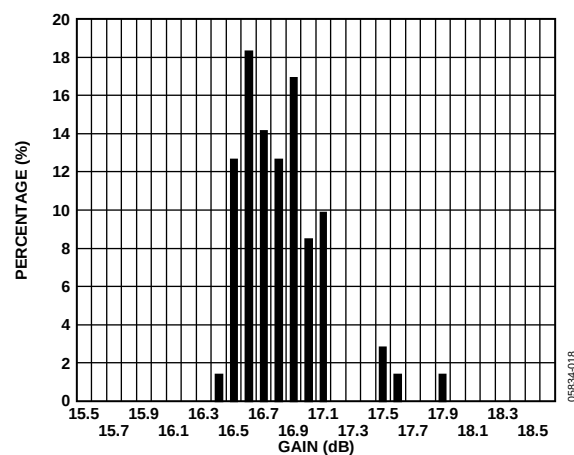
Figure 19. Gain Distribution at 190 MHz, VPOS = 5 V
