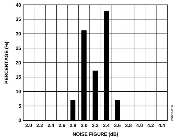
Figure 20. Noise Figure Distribution at 190 MHz, VPOS = 5 V
