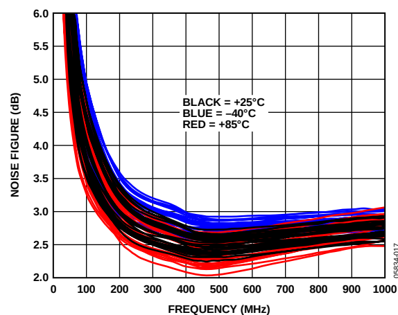
Figure 18. Noise Figure Temperature Distribution, VPOS = 5 V
