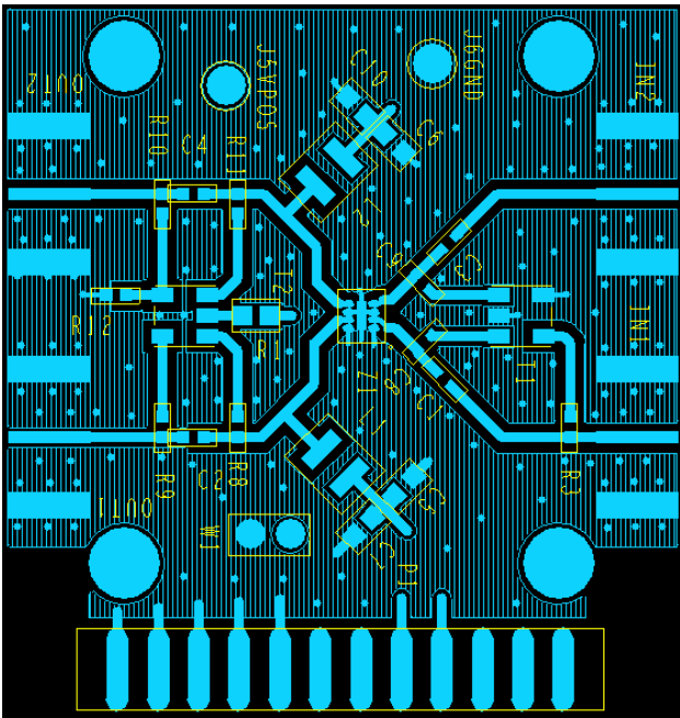
Figure 26. Evaluation Board Layout
