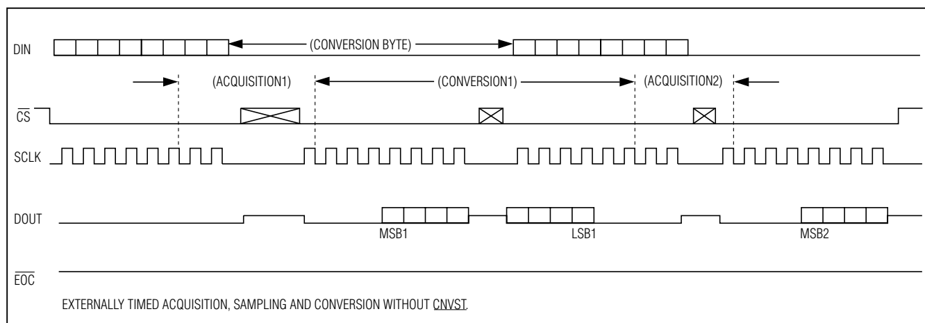
Figure 7. Clock Mode 11
