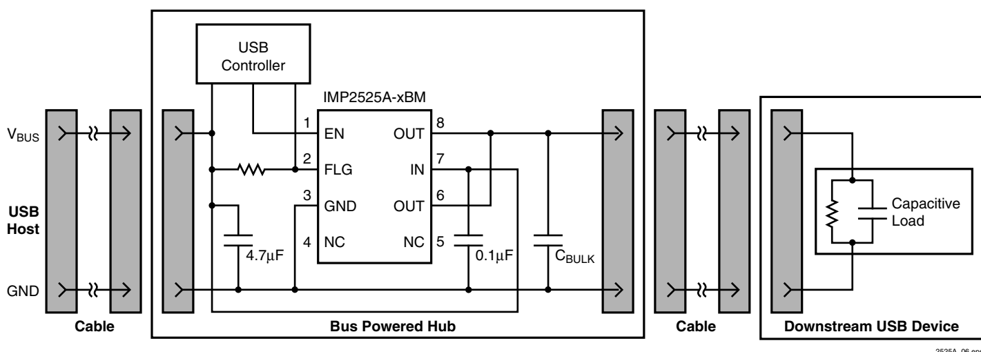
Figure 2. Soft-Start Application
