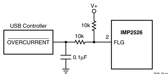
Figure 4. Transient Filter
