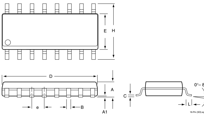
SO (16-Pin)
