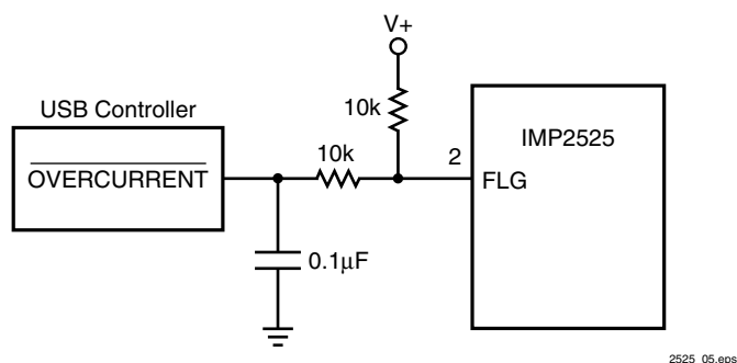
Figure 4. Transient Filter
