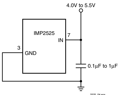
Figure 1. Supply Bypassing
