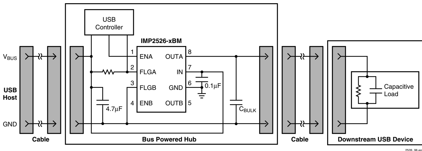
Figure 2. Soft-Start Application
